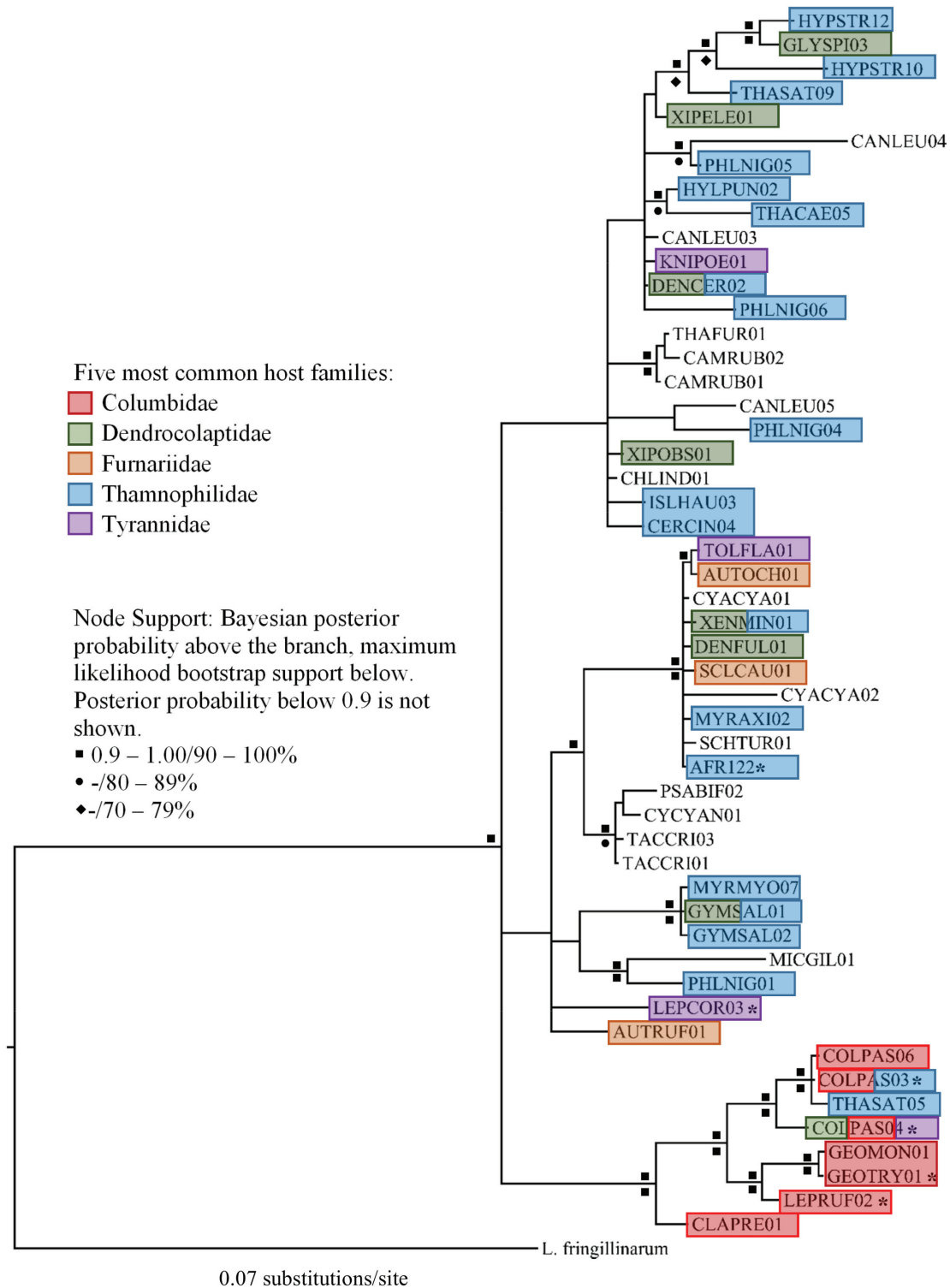
Figure 3. Phylogenetic reconstruction of Amazonian Haemoproteus lineages. Previously reported lineages (MalAvi) are indicated with an asterisk. The five most common host families are indicated by colored blocks.
